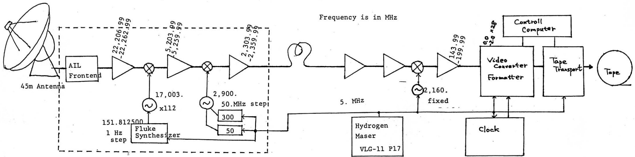
45m Radiotelescope Frequency Diagram for 22GHz MkIII VLBI Experiment Feb. 5, 1984.
