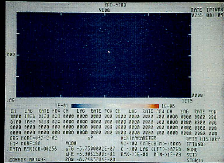
3C454.3 (22 GHz continuum)
